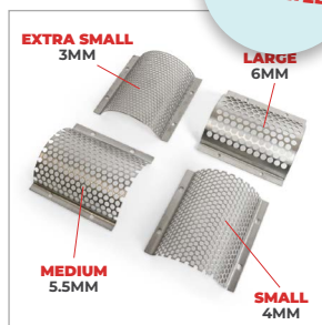
FOUR DIFFERENT PARTICLE SCREEN SIZES AVAILABLE
